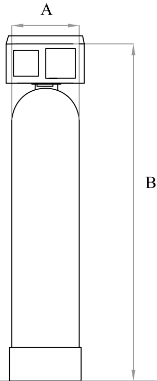
FRONT VIEW -MINERAL TANK
